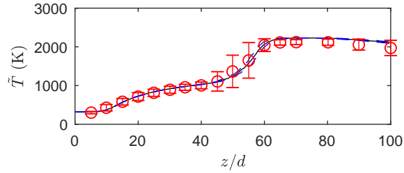
Figure 2: Centerline Favre-average temperature. As per Fig. 1.
