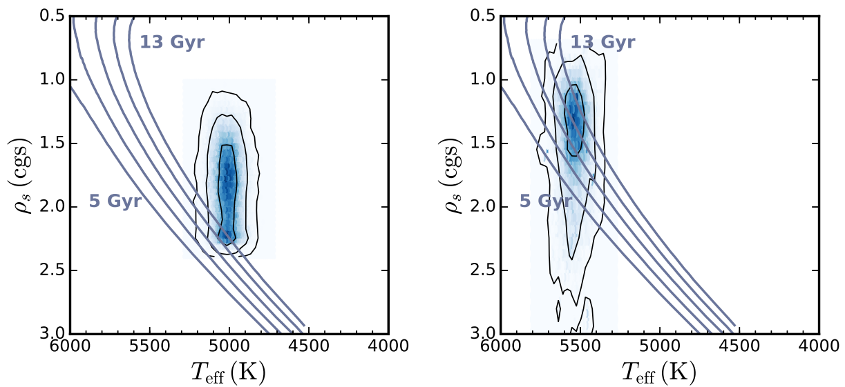
Fig. 6.— Stellar parameters are derived via interpolation of the Dartmouth isochrones. The stellar density ( \rho_s ), derived from the transit light curve, and the spectroscopic effective temperature T_{\text{eff}} and metallicity [\text{Fe}/\text{H}] are compared against isochrone tracks at each MCMC iteration to constrain the stellar properties. The stellar densities and effective temperatures of K2-114 (left) and K2-115 (right) are plotted. The Dartmouth solar metallicity isochrones at ages of 5, 7, 9, 11, and 13 Gyrs are drawn as a guide. Note that solutions yielding ages > 13 Gyr are removed during the derivation of system and stellar parameters in the global analysis, as that age is older than the age of the thin disk of the galaxy.
