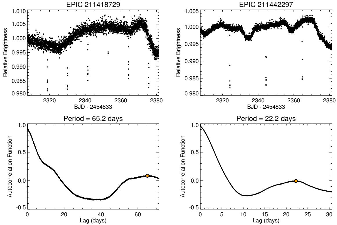
Fig. 3.— K2-114 (left) and K2-115 (right) K2 light curves without detrending (top panels), and the light curve’s autocorrelation (bottom panels) where the strongest peak is marked by an orange circle, and the period is listed in the panels’ title. The in-transit photometric data was removed while calculating the autocorrelation function. For K2-114 the 65.2 day periodicity identified through the autocorrelation is close to the K2 data time span. At such time scales it is difficult to separate between stellar variability and systematic features in K2 data, hence we claim a detection of the rotation period only for K2-115 where the 22.2 day variability is identified visually in the light curve. We estimate a 10 % uncertainty on that rotation period due to differential rotation.
