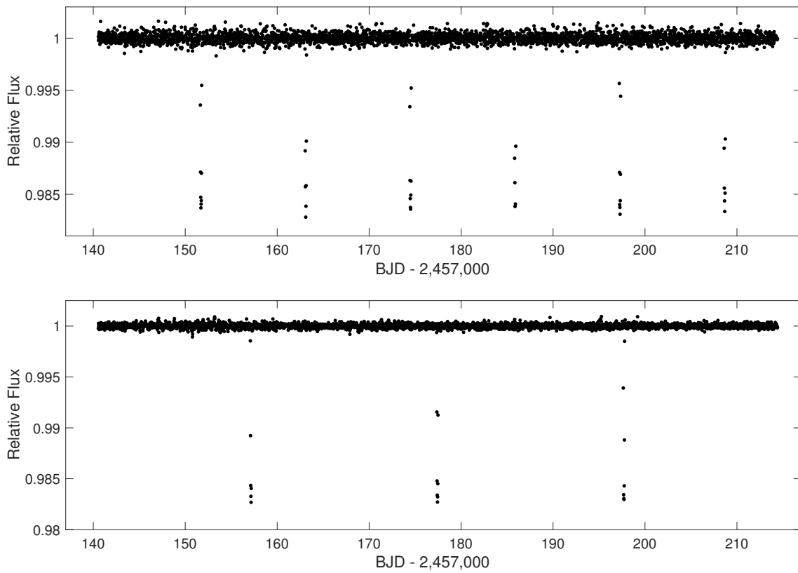
Fig. 1.— Complete, detrended, and normalized K2 Campaign 5 light curves of K2-114 (top), including 6 transit events, and of K2-115 (bottom), including 3 transit events.
