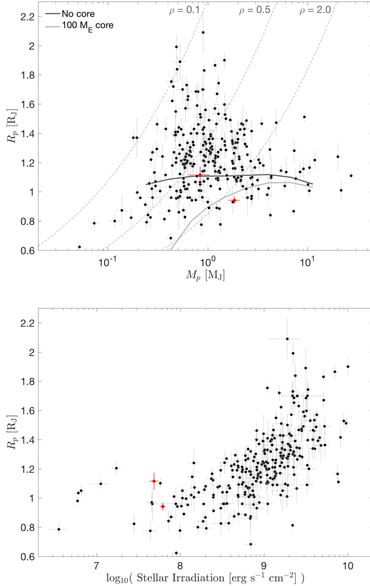
Fig. 7.— Figures show the planet radius (linear scale) as a function of planet mass (log scale; top panel) and stellar irradiation (log scale; bottom panel). K2-114b and K2-115b are marked in red. In the top panel the solid lines encompass the theoretically expected region where planets are expected to reside in this parameter space (Fortney et al. 2007), between a core-less planet (solid black line) and a planet with a massive core of 100 M_{\oplus} (solid gray line). Both theoretical curves are for an assumed orbital star-planet separation of 0.045 au, although the planet radius changes by up to only \approx 10\% between a separation of 0.02 au and 0.10 au (Fortney et al. 2007). The dashed gray lines mark lines of equal mean density, and the density is labeled in the top part of the panel, in units of \text{g cm}^{-3} . Both panels show in black 273 planets with R_p over 0.6 R_J , planet radius error below 0.15 R_J , and planet mass error below 20% of the planet mass itself, to include only planets with well measured mass and radius. Circumbinary planets and directly imaged planets are excluded from these plots. Data shown in these plots was taken from the NASA Exoplanet Archive (Akeson et al. 2013) on 2017 June 1st.
