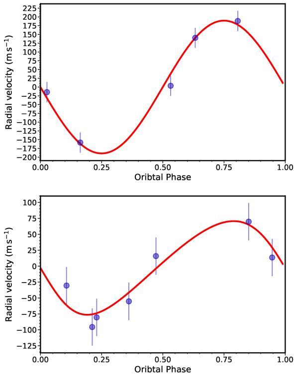
Fig. 5.— Phase folded Keck/HIRES RV curves of K2-114 (top) and K2-115 (bottom). RVs are marked in blue circles and error bars and the fitted model is marked in a red solid line. The error bars shown in the plots include the jitter term added in quadrature (see Sec. 4).
