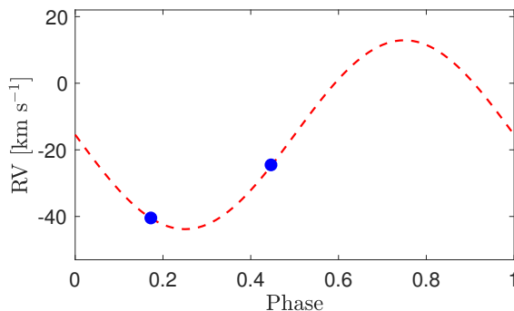
Fig. 9.— Euler/CORALIE RVs of EPIC 212504617 phase folded at the transit period of P=39.26 day. RVs are marked in blue (error bars are smaller than the markers size), and the dashed line shows the best fit e=0 orbital solution. Phase zero is the primary eclipse (transit) phase. The fitted semi-amplitude is 28.4 \text{ km s}^{-1} . Since this is a two-parameter model fitted to two RVs this model is used only as an estimate for the orbital RV variation. This estimate rules out the possibility of a sub-stellar mass companion, as discussed in more details in the text.
