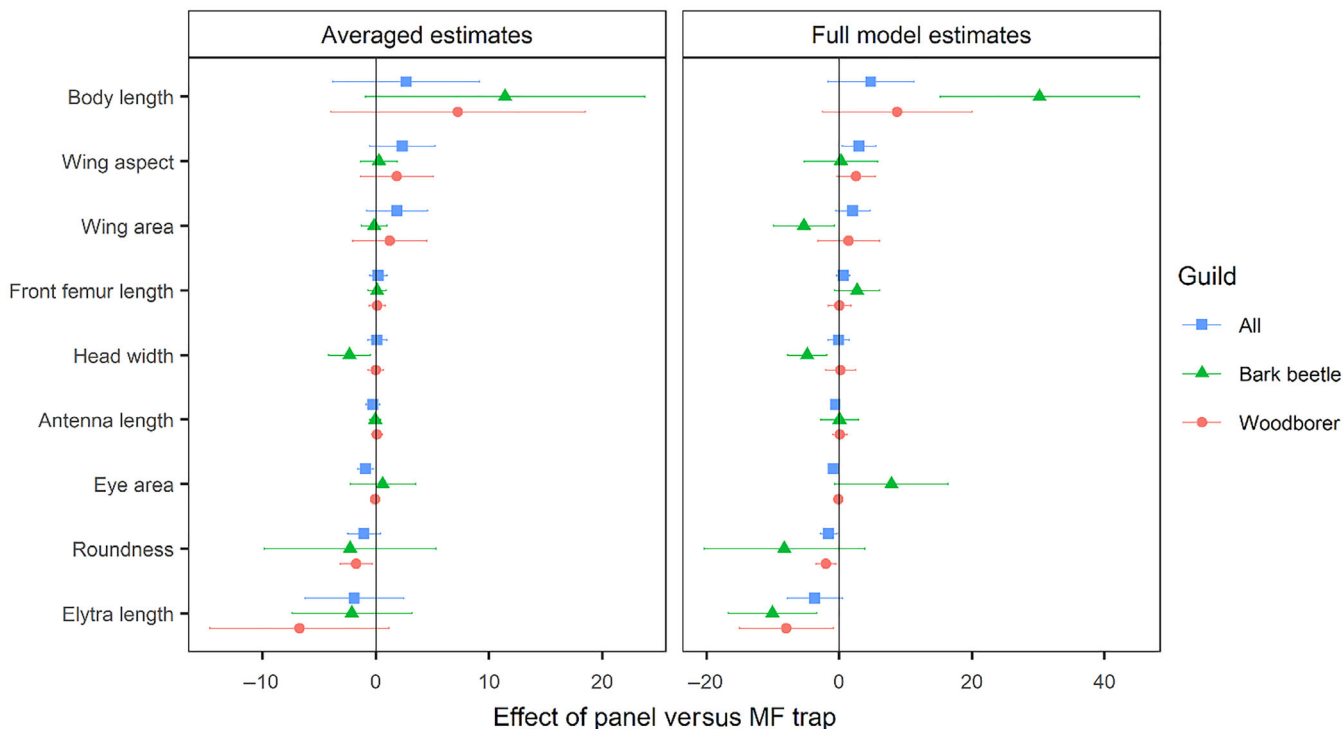
FIGURE 2 Influence of morphological traits on capture rates in panel versus multiple-funnel (MF) traps, separated by the two major coleopteran guilds, where x-axis values >0 represent higher capture rates in panel compared with MF traps. Points show mean effect sizes, with bars representing 95% CIs. Averaged estimates are derived from models with all possible combinations of traits using an information theoretic approach, whereas the full model includes all traits.
