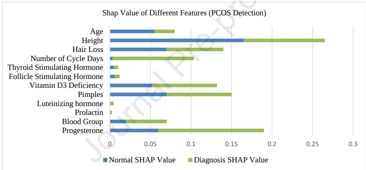
Figure 8. Features importance using SHAP value
