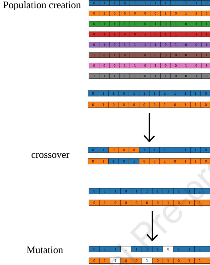
Figure 3. The main process of GA
