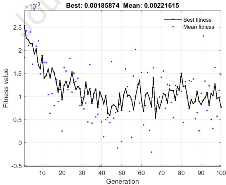
Figure 5. The Optimal Fitness Value
