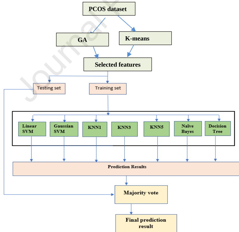
Figure 4. The proposed ensemble model.
