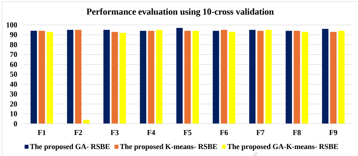
Figure 7. Evaluation using 10-fold cross-validation.
