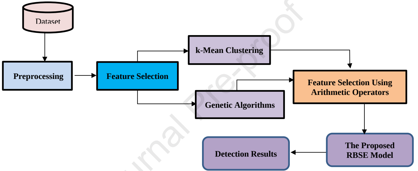
Figure 1. Block diagram of the proposed method.
