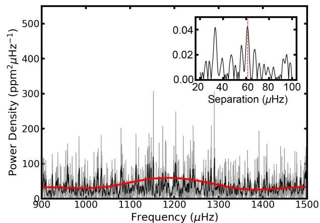
Figure 6. Power spectrum of the Sector 3 TASOC light curve of TOI-257 (grey line). The black and red lines show the power spectrum smoothed with a boxcar width of 2 \mu\text{Hz} and Gaussian with a full width at half max of \Delta\nu = 61.4 , respectively. The inset shows the autocorrelation of the power spectrum, with a red line marking the expected value of \Delta\nu based on the location of the power excess.
