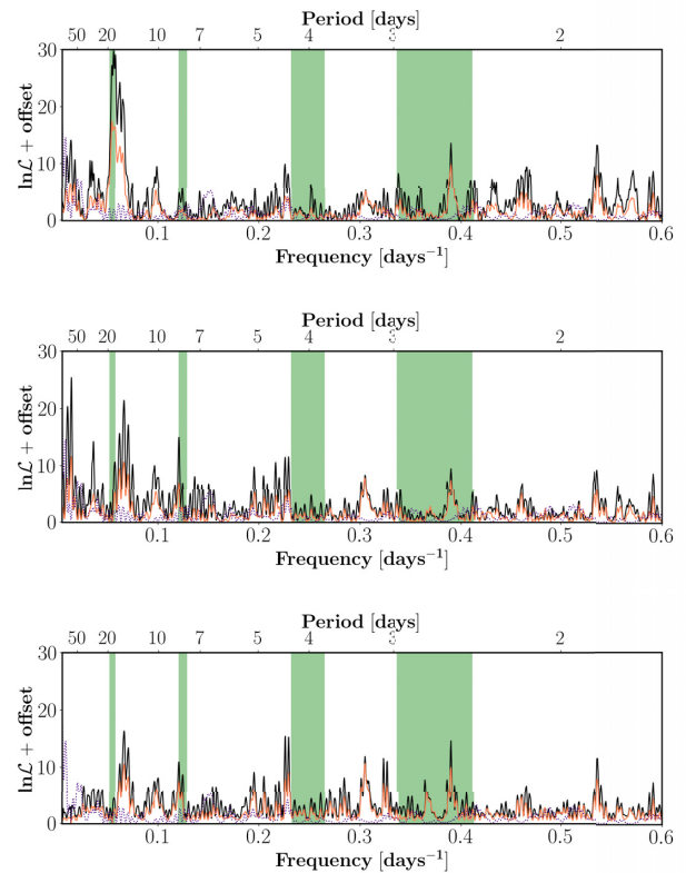
Figure 14. Log-likelihood periodograms as a function of frequency generated using RadVel. Shaded from left to right are the frequency of planet b (insignificant width), the estimated stellar rotation frequency 1/P_{\text{rot}} from Table 5 (width is \pm 1\sigma ), and harmonics 2/P_{\text{rot}} , 3/P_{\text{rot}} . The orange line includes a Gaussian process (GP) to model stellar activity with a quasi-periodic kernel with priors listed in Table 5, while the black line models remaining jitter as per-instrument Gaussian noise. The dashed line represents the window function (arbitrary scaling). Top: A one-planet circular model tested at a wide range in fixed periods, fitting for K , T_c and the relative instrument dependent offsets and noise terms (or single GP). Middle: Same, but for a two-planet model assuming a fixed period and T_c for planet b from Table 4, but varying both semi-amplitudes to search for additional planets. Bottom: Same as middle, but searching for a third planet such that P_c \sim \mathcal{N}(71.5, 1) . We see no evidence for additional periodic variations in the RVs past 18 days over the full observing window.
