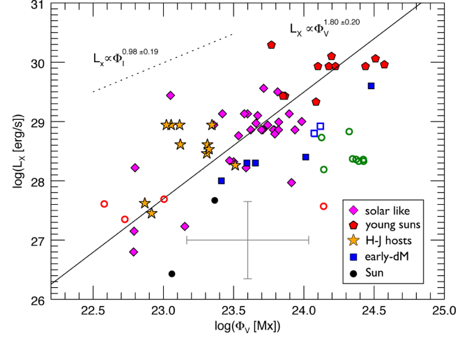
Figure 5. Correlation between X-ray luminosity L_X and large-scale magnetic flux ( \Phi_V = 4\pi R_*^2 \langle|B_V|\rangle ) derived from the ZDI technique for the non-accreting stars in our sample. The open symbols are as in Fig. 3 and were not considered in the fit (solid line). The dotted line, at an arbitrary vertical offset, is indicative of the slope found from ZB measurements for dwarf stars between L_X and \Phi_I = \langle|B_I|\rangle 4\pi R_*^2 (Pevtsov et al. 2003). These slopes are consistent with each other within 3\sigma , but samples with a large dynamic range of ( \langle|B_I|\rangle ) are desirable to better constrain this result (see text).
