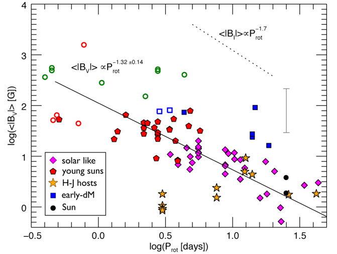
Figure 3. Correlation between the average large-scale field strength derived from the ZDI technique ( \langle |B_V| \rangle ) and rotation period P_{\text{rot}} , for the non-accreting stars in our sample. Our data support the presence of a linear-type dynamo for the large-scale field (i.e. \langle |B_V| \rangle \propto \Omega_* \propto P_{\text{rot}}^{-1} ) within 3\sigma , although a large scatter exists. The open symbols (not considered in the fit) are saturated M dwarf stars without age estimates: blue squares for M_* \geq 0.4 M_\odot (early Ms), green circles for 0.2 < M_*/M_\odot < 0.4 (mid Ms) and red circles for M_* \leq 0.2 M_\odot (late Ms). The dotted line, at an arbitrary vertical offset, is indicative of the slope found from ZB measurements between \langle |B_V| \rangle and P_{\text{rot}} (Saar 1996).
