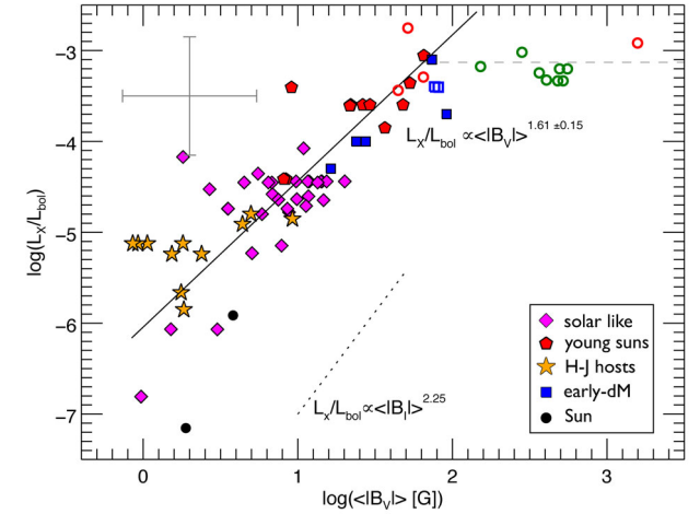
Figure 6. Correlation between the ratio of X-ray-to-bolometric luminosity ( L_X/L_{bol} ) and large-scale magnetic field derived from the ZDI technique ( \langle|B_V|\rangle ) for the non-accreting stars in our sample. The open symbols are as in Fig. 3 and were not considered in our fit (solid line). The dashed line indicates the saturation plateau for Ro \lesssim 0.1 at \log(L_X/L_{bol}) \approx -3.1 (Wright et al. 2011). The dotted line, at an arbitrary vertical offset, is indicative of the slope found from ZB measurements (derived from results by Saar 2001; Wright et al. 2011).
