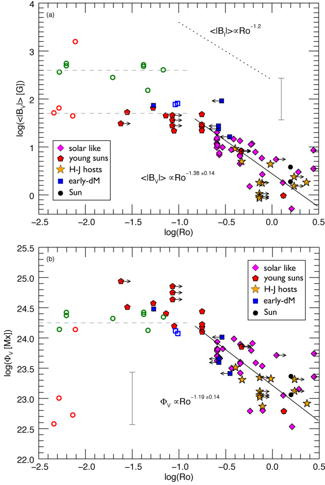
Figure 4. (a) Correlation between the average large-scale field strength derived from the ZDI technique ( \langle|B_V|\rangle ) and Rossby number Ro , for the non-accreting stars in our sample. Using Stokes I data, Reiners et al. (2009) showed that ( \langle|B_I|\rangle ) saturates for Ro \lesssim 0.1 . Donati et al. (2008c) suggested that there might be two different levels of saturation (dashed lines) among the low-mass stars, caused by different efficiencies at producing large- and small-scale fields. (b) Same as in (a), but now considering the magnetic flux \Phi_V . Note that the bi-modality in the saturation level is removed if \Phi_V is considered instead of ( \langle|B_V|\rangle ). Open symbols are as in Fig. 3. Solid lines show power-law fits considering objects with Ro \gtrsim 0.1 . The dotted line (arbitrary vertical offset) in the upper panel is indicative of the slope found from ZB measurements between ( \langle|B_I|\rangle ) and Ro (Saar 2001).
