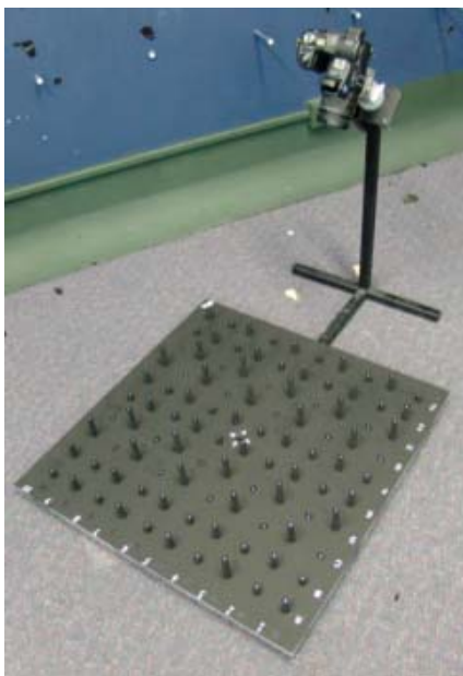
Figure 2 Three-dimensional camera calibration device
