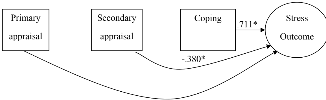
Figure 1: 3-path model (Model 1) for male samples
